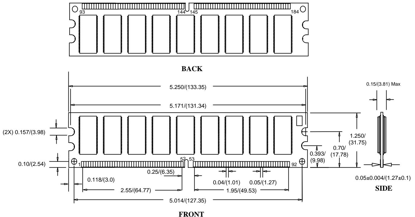
Figure 1: 3AMD1400-1GB-R 184-Pin SDRAM Module
